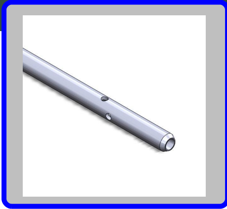
AS-5438201-10 TUBE, SIPHON, VIB WATER COOL 72" OAL 78 7/8"
