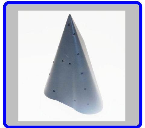
AS-5463625-MOD CERAMIC FORMER NOSE IMPROVED AIR FLOW REPLACES AS-5463625
