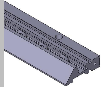
AS-5618268 57" PLATE LOCKUP BAR CURRENT STYLE OAL 57.201"
