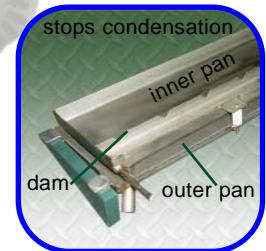
Double Wall Water Pan (DWWP)
