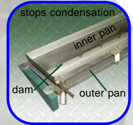
Double Wall Water Pan (DWWP)
